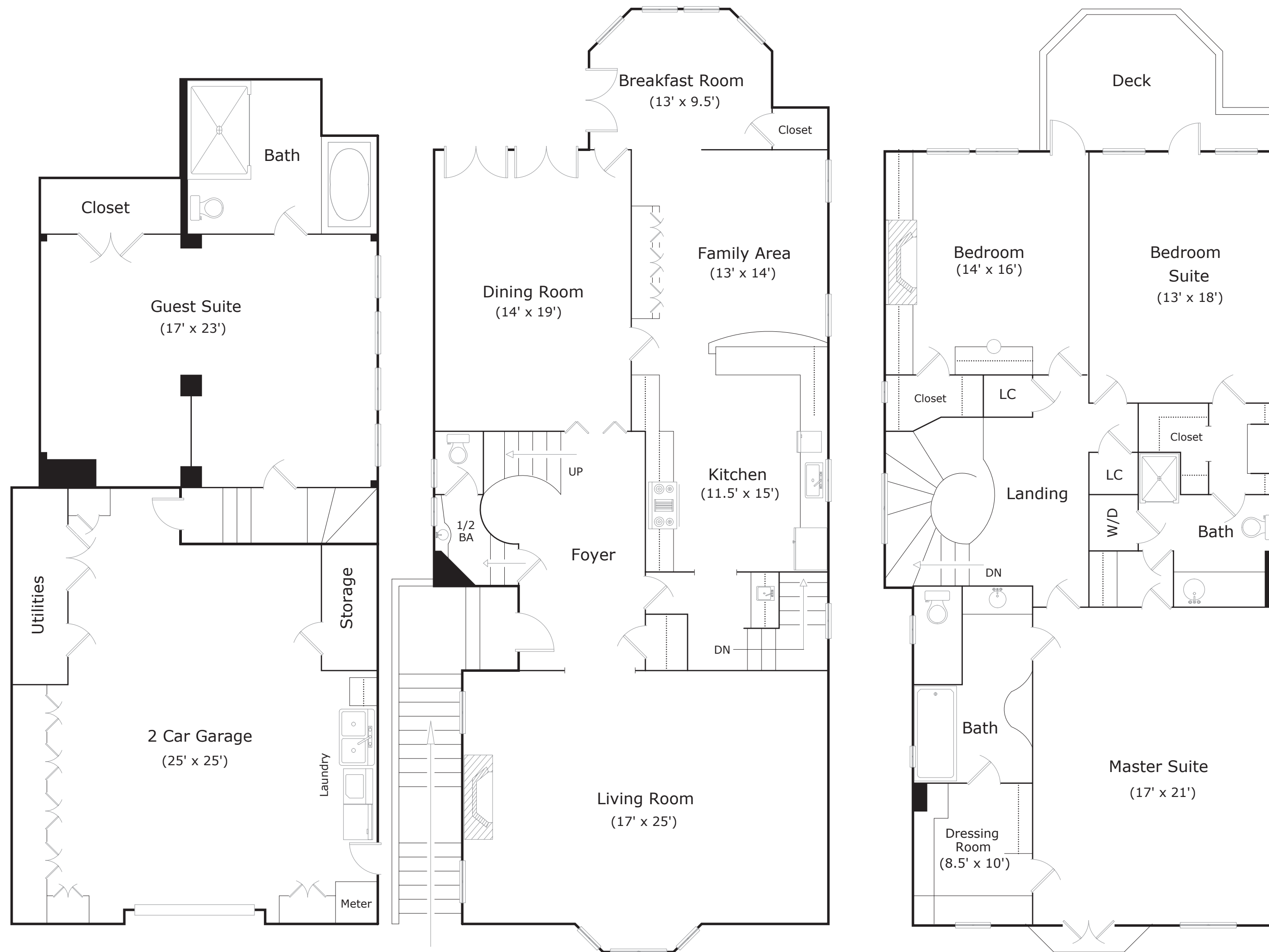
FIRST FLOOR
